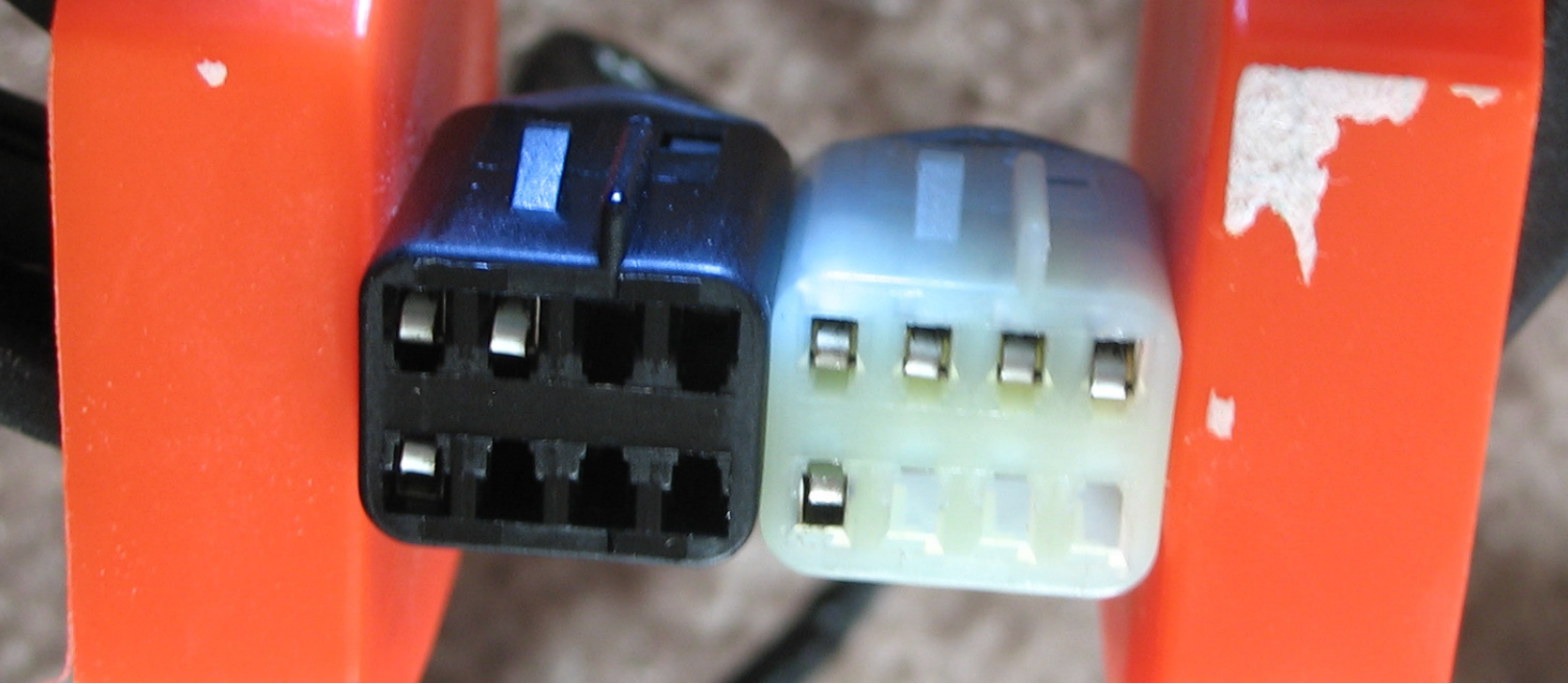
2012 Camaro Outside Mirror Connectors - Passenger's Side Shown Black - Unheated • White - Heated • Same Exact Size
