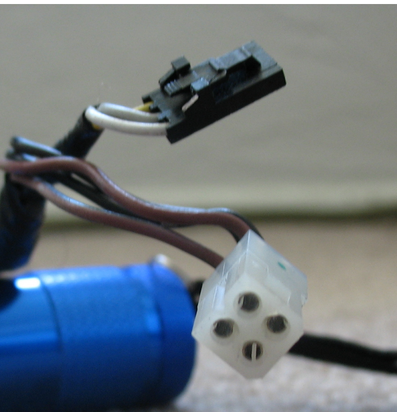
2012 Camaro Outside Mirror Connectors - Driver's Side Shown Black Mirror Motor Connector • White 4-Pin Connector to Heated Mirror Back
