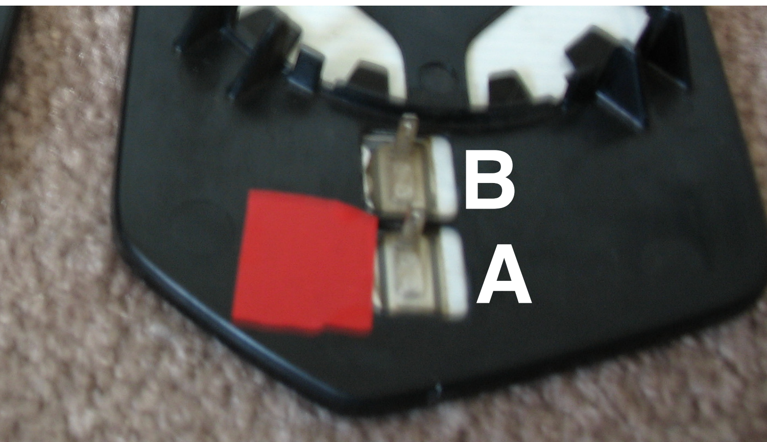
2012 Camaro Outside Heated Mirrors - Back Side Shown Passenger's Side shows 2 Single Pin Connectors - same as C-D above
