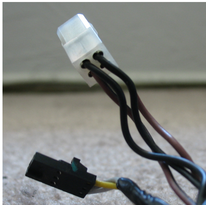
2012 Camaro Outside Mirror Connectors - Driver's Side Shown Black Mirror Motor Connector • White 4-Pin Connector to Heated Mirror Back
