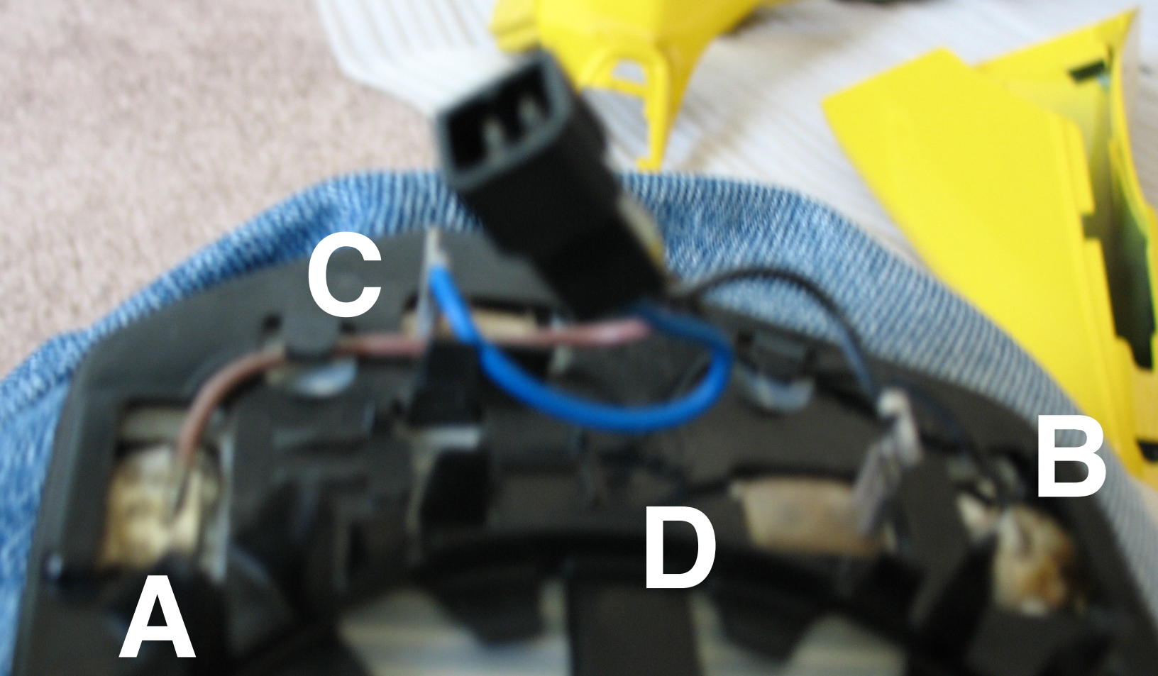
2012 Camaro Outside Heated Mirrors - Back Side Shown Driver's Side shows 4 wires into 4-Pin Connector
