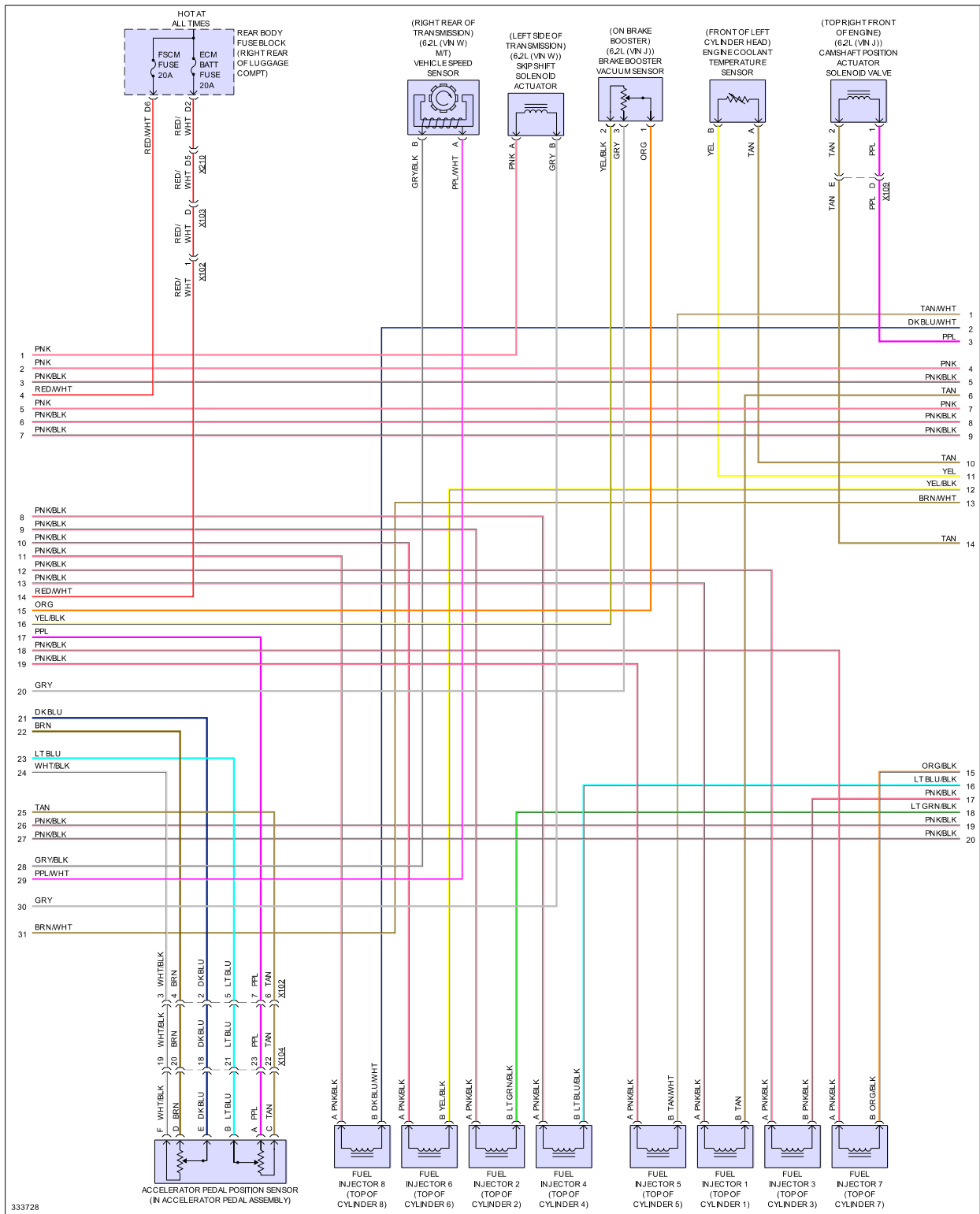
Fig 3: 6.2L VIN W, Engine Performance Circuit (3 of 6)
