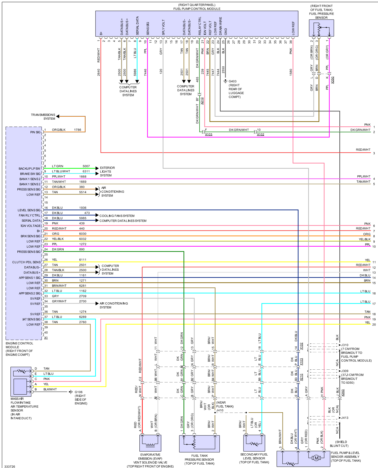
Fig 1: 6.2L VIN W, Engine Performance Circuit (1 of 6)
