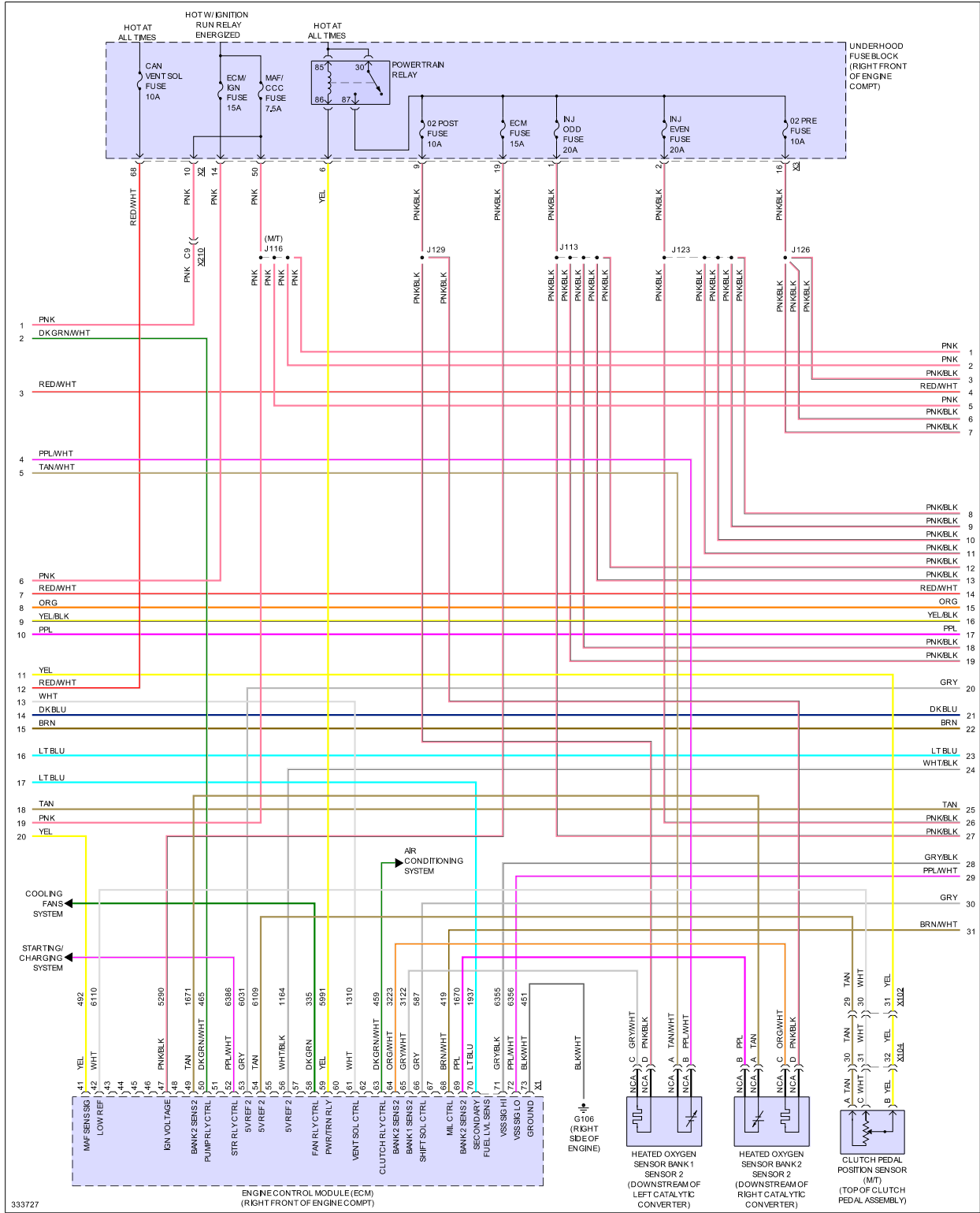
Fig 2: 6.2L VIN W, Engine Performance Circuit (2 of 6)
