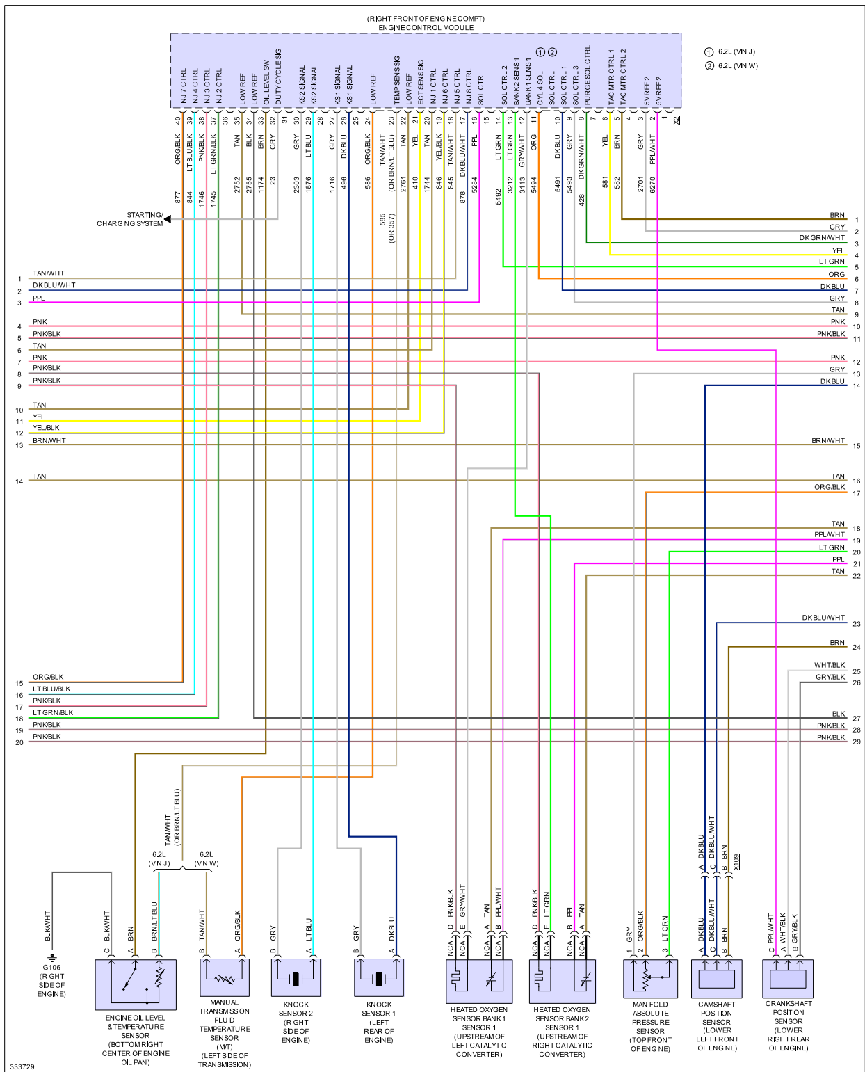
Fig 4: 6.2L VIN W, Engine Performance Circuit (4 of 6)
